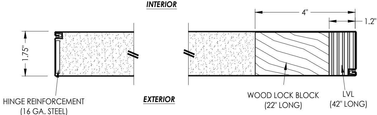
3 2 HORIZONTAL CROSS SECTION
