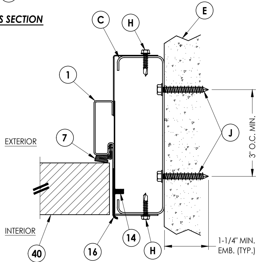
4 HORIZONTAL CROSS SECTION Steel Stud Construction
